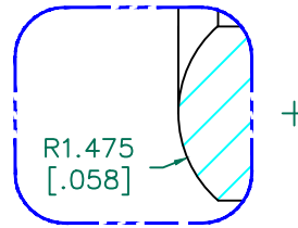
DETAIL "A" CHAMFER SCALE=10:1
